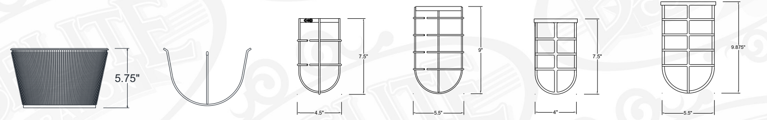
REF 9.5" DIAMETER REFRACTOR UGR U WIRE GRILL WG-1 WIRE GUARD WG-2 WIRE GUARD Available for shades 12" or higher GU-1 CAST ALUMINUM GUARD GU-2 CAST ALUMINUM GUARD Available for shades 12" or higher
