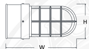
BSM4 H - 6.25" W - 10.75" BSM14 H - 6.25" W - 12.75"
