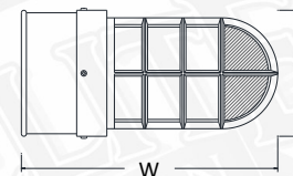
BSM5 H - 6.25" W - 10.75" BSM15 H - 6.25" W - 12.75"
