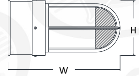
BSM2 H - 6.25" W - 10.75" BSM12 H - 6.25" W - 12.75"
