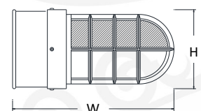
BSM6 H - 6.25" W - 10.75" BSM16 H - 6.25" W - 12.75"
