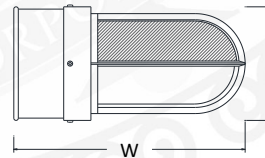
BSM3 H - 6.25" W - 10.75" BSM13 H - 6.25" W - 12.75"
