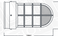
BSM5 H - 6.25" W - 9.25" BSM15 H - 6.25" W - 11.25"
