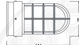
BSM4 H - 6.25" W - 9.25" BSM14 H - 6.25" W - 11.25"
