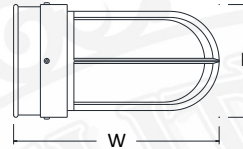
BSM1 H - 6.25" W - 9.25" BSM11 H - 6.25" W - 11.25"
