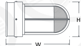
BSM2 H - 6.25" W - 9.25" BSM12 H - 6.25" W - 11.25"
