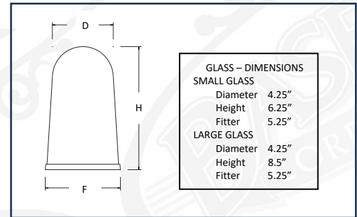
FR FROSTED LARGE GLASS
