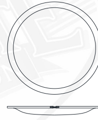
CRL13 13" CURVED POLYCARB LENS CRL17 17" CURVED POLYCARB LENS
