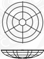
GR11 11" WIRE GRILL GR13 13" WIRE GRILL GR17 17" WIRE GRILL
