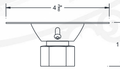
SLC 1/2" SLOPE CEILING CANOPY 1/2"
