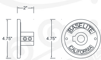
CB 1/2" CAST ALUMINUM BACKPLATE 1/2 NPT
