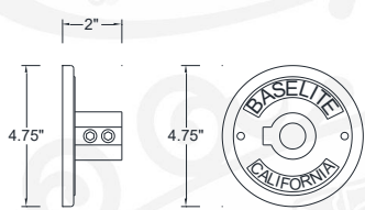
CB 1/2" CAST ALUMINUM BACKPLATE 1/2 NPT
