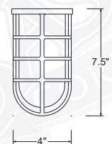
GU-1 CAST ALUMINUM GUARD
