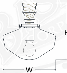
SCP.SHC14 H-14.5" W-14"
