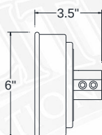
LWTM WEATHERTIGHT CF WALL MOUNT
