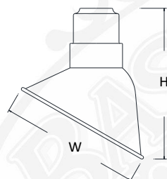
A810 H - 10.75" W - 10"
