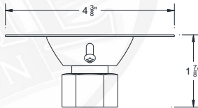
SLC 1/2" SLOPE CEILING CANOPY 1/2" *(Slopes To 20 Degrees)
