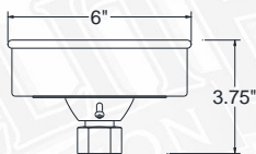
LSLC - LED SLOPE CEILING CANOPY 1/2" *(Slopes To 20 Degrees)
