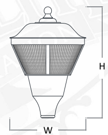
INT20 H-28" W-20" F-3"
