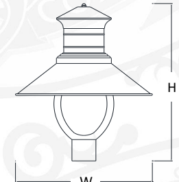
IMC20 H-22" W-20" F-3"
