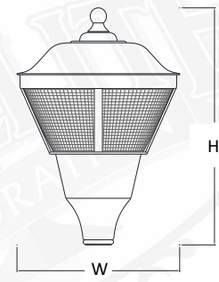
INT20 H-28" W-20" F-3"
