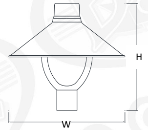
IL202 H-16.5" W-20" F-2 3/8" IL203 H-18.5" W-20" F-3" IL262 H-16.5" W-26" F-2 3/8" IL263 H-18.5" W-26" F-3"
