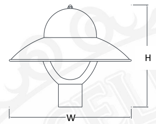
IM18 H-16.5" W-18" F-3" IM20 H-16.5" W-20" F-3"
