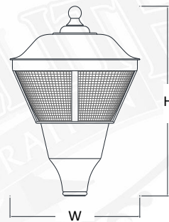
INT20 H-28" W-20" F-3"
