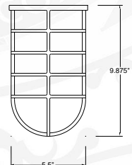
GU-2 CAST ALUMINUM GUARD
