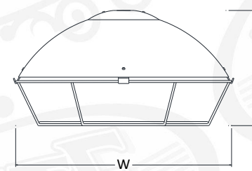
QD20 H-10 ½" W-21" *EFGR COMES STANDARD WITH SHADE. ALL OTHER ACCESSORIES DO NOT APPLY
