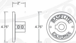
CB 1/2" CAST ALUMINUM BACKPLATE 1/2 NPT
