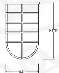
GU-2 CAST GUARD
