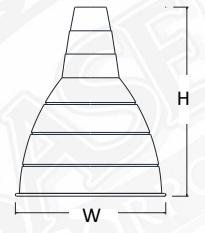
CO15 H-19" W-15"
