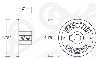
CB 1/2" CAST ALUMINUM BACKPLATE 1/2 NPT CB 3/4" CAST ALUMINUM BACKPLATE 3/4 NPT
