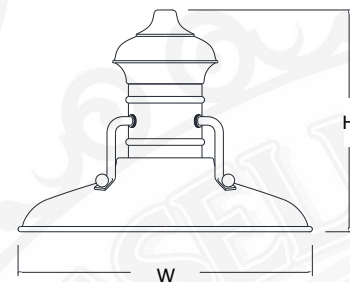
TAR14 H-10.5" W-14" TAR16 H-10.5" W-16" TAR18 H-11.5" W-18"
