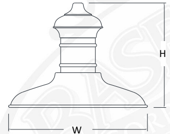
TA12 H-10.5" W-12" TA14 H-10.5" W-14" TA16 H-10.5" W-16" TA18 H-11.5" W-18"
