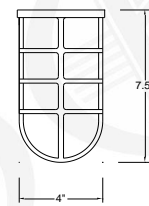
GU-1 CAST ALUMINUM GUARD
