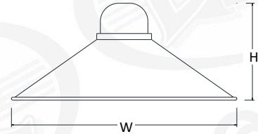
WE14 H-6" W-14" WE18 H-8" W-18.5"
