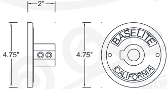
CB 1/2" CAST ALUMINUM BACKPLATE 1/2 NPT CB 3/4" CAST ALUMINUM BACKPLATE 3/4 NPT
