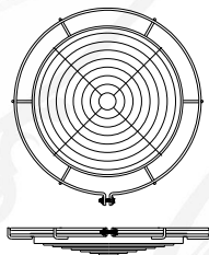
LGR16 16" LOUVERED GRILL
