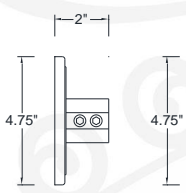
CB 1/2" CAST ALUMINUM BACKPLATE 1/2 NPT CB 3/4" CAST ALUMINUM BACKPLATE 3/4 NPT
