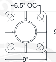
Template for Square Poles
