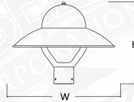
IM18 H-14.5" W-18" F-3"
