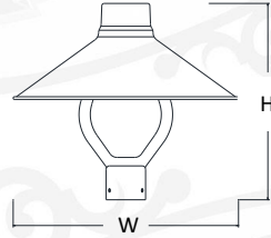
IL202 H-17" W-20" F-2 3/8"
