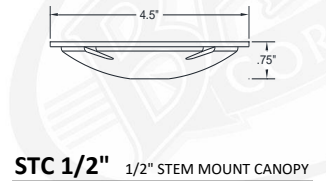
STC 1/2" 1/2" STEM MOUNT CANOPY
