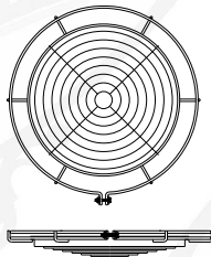
LGR18 18" LOUVERED GRILL
