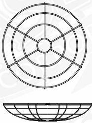
GR18 18" WIRE GRILL
