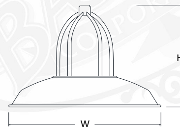
URW16 H-12" W-16" URW18 H-12" W-18" URW20 H-15.5" W-20"
