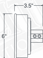
CFWTM WEATHERTIGHT CF WALL MOUNT
