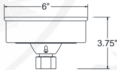
LSLC 1/2" LED SLOPE CEILING CANOPY
