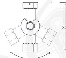
LGSWL 1/2" NPT SWIVEL
