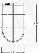
WG1 WIRE GUARD
