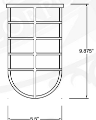
GU-2 CAST GUARD Available for shades 12" or higher
