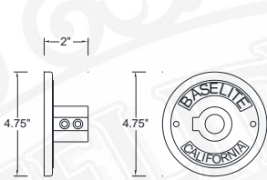
CB 1/2" CAST ALUMINUM BACKPLATE 1/2 NPT CB 3/4" CAST ALUMINUM BACKPLATE 3/4 NPT
