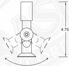
SWL 1/2" NPT SWIVEL
