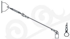
TRB 1/2"-4' Cable SUPPORT
