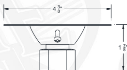
SLC 1/2" SLOPE CEILING CANOPY 1/2"
