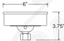
LSLC 1/2" SLOPE CEILING CANOPY 1/2" LSLC 3/4" SLOPE CEILING CANOPY 3/4" (Slopes to 20 Degrees)
