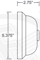
CBC 1/2" 1/2" BACKPLATE COVER CBC 3/4" 3/4" BACKPLATE COVER * Includes slip ring to hold 1/2" or 3/4" arm extension
